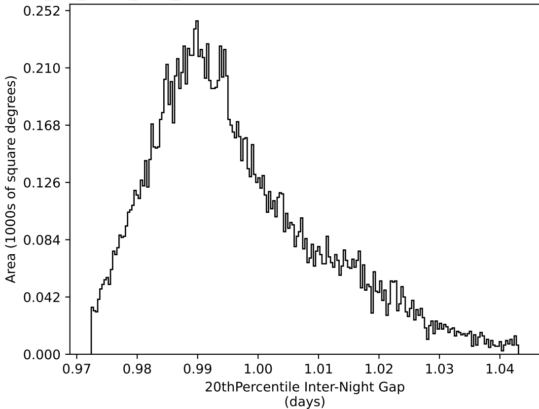
mw_roll_bulge_v3.3_10yrs WFD all bands: 20thPercentile Inter-Night Gap
