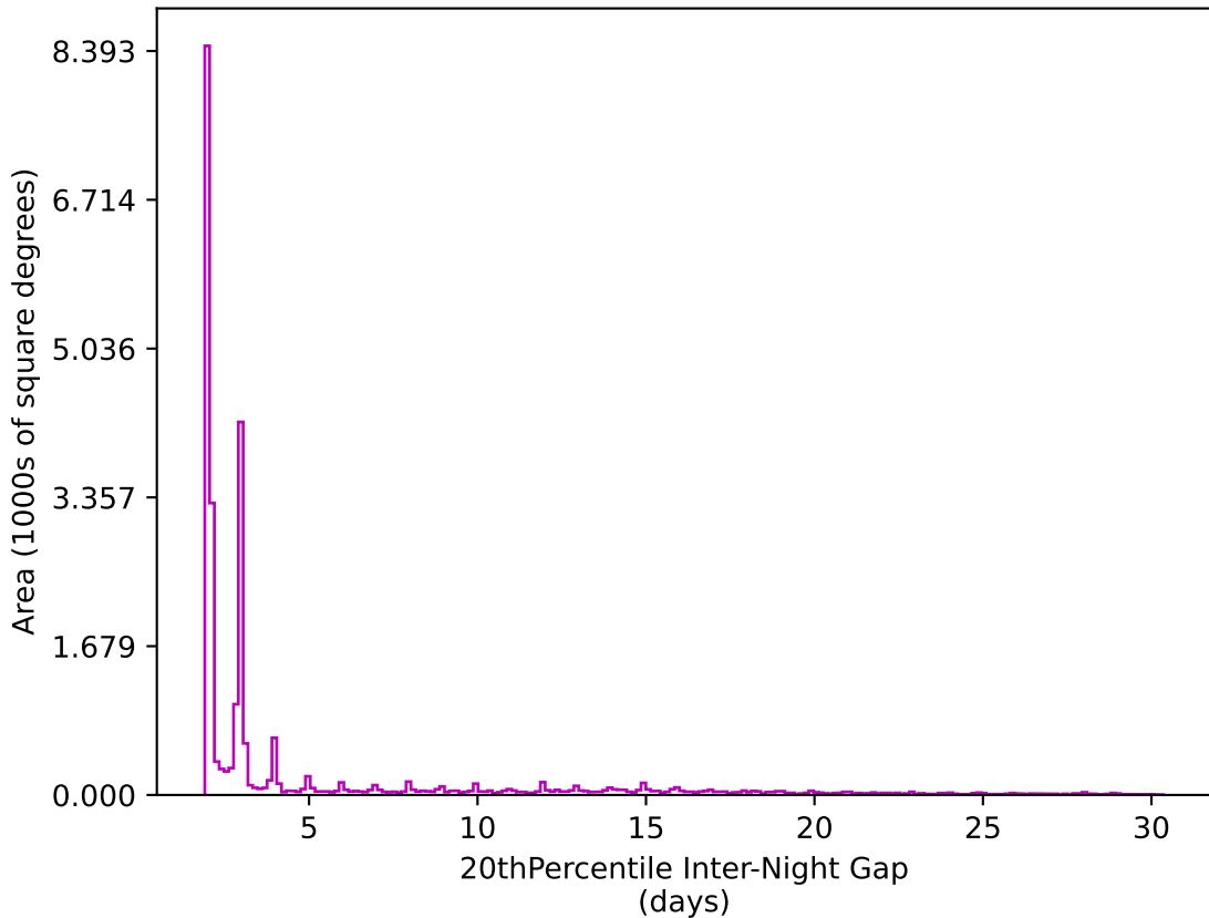
mw_roll_bulge_v3.3_10yrs All sky z band: 20thPercentile Inter-Night Gap
