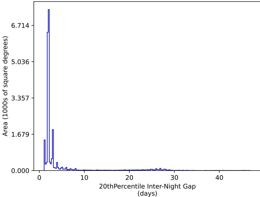
mw_roll_bulge_v3.3_10yrs All sky y band: 20thPercentile Inter-Night Gap
