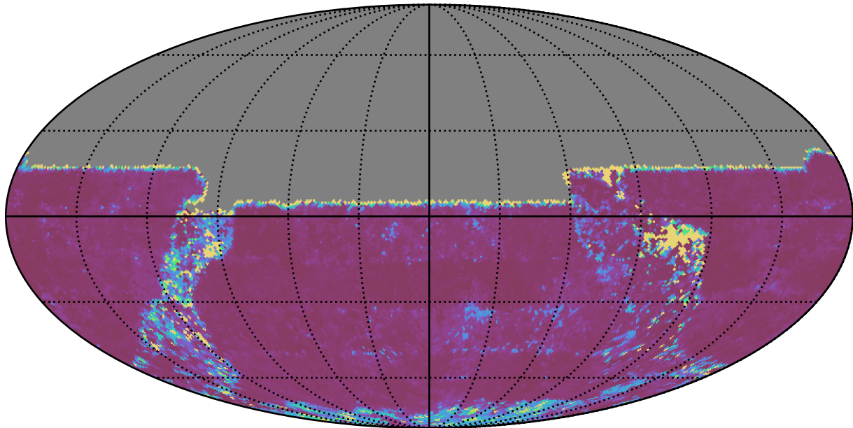
mw_roll_bulge_v3.3_10yrs All sky u band: 20thPercentile Inter-Night Gap
