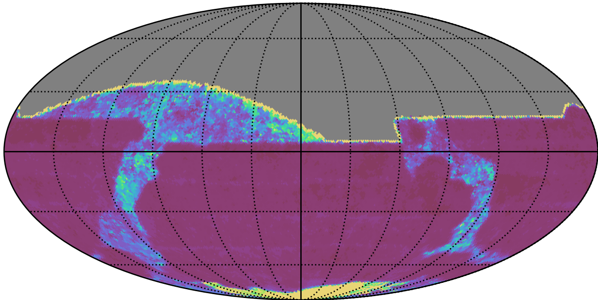
mw_roll_bulge_v3.3_10yrs All sky r band: 20thPercentile Inter-Night Gap
