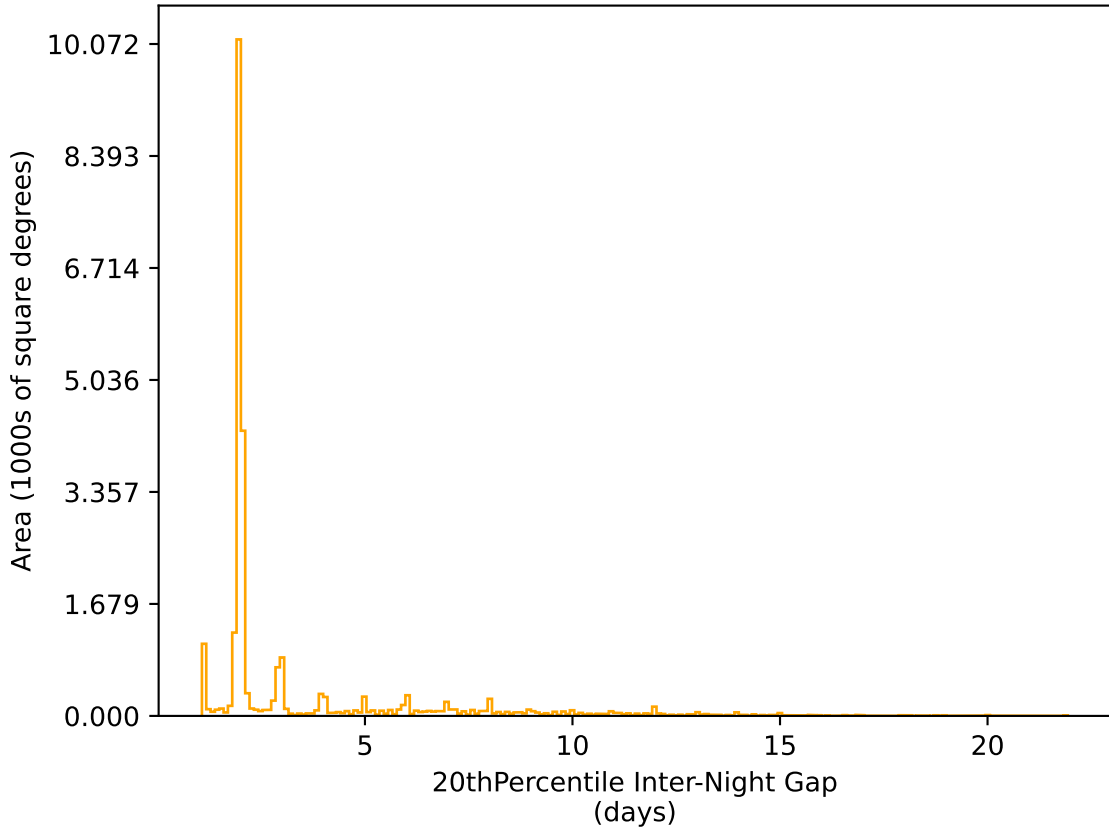
mw_roll_bulge_v3.3_10yrs All sky r band: 20thPercentile Inter-Night Gap
