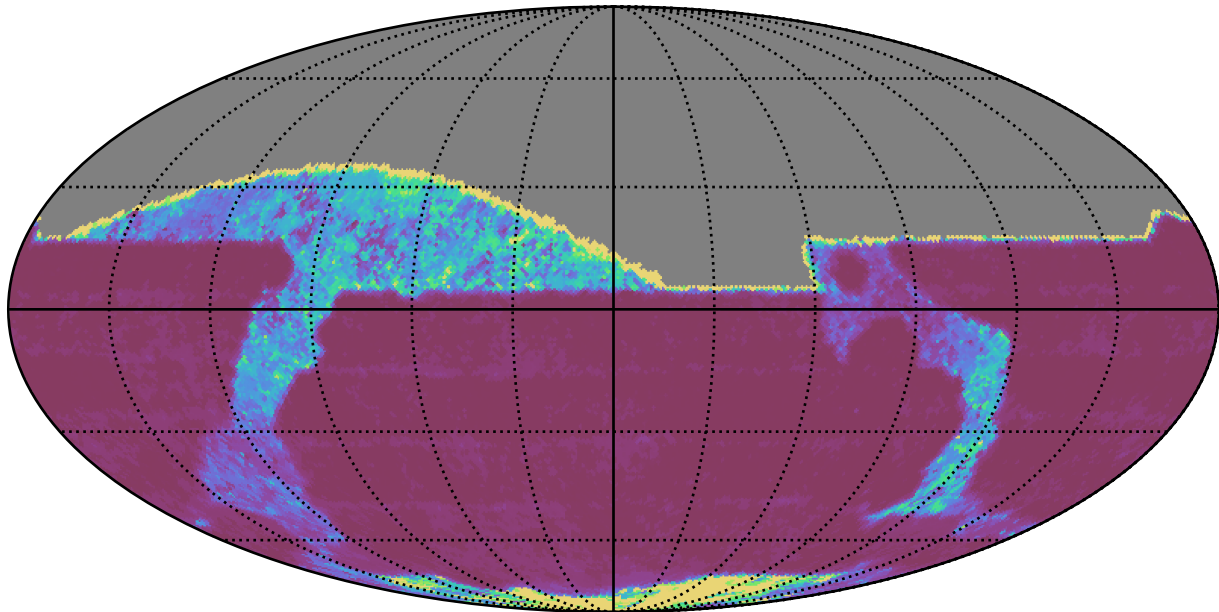
mw_roll_bulge_v3.3_10yrs All sky i band: 20thPercentile Inter-Night Gap
