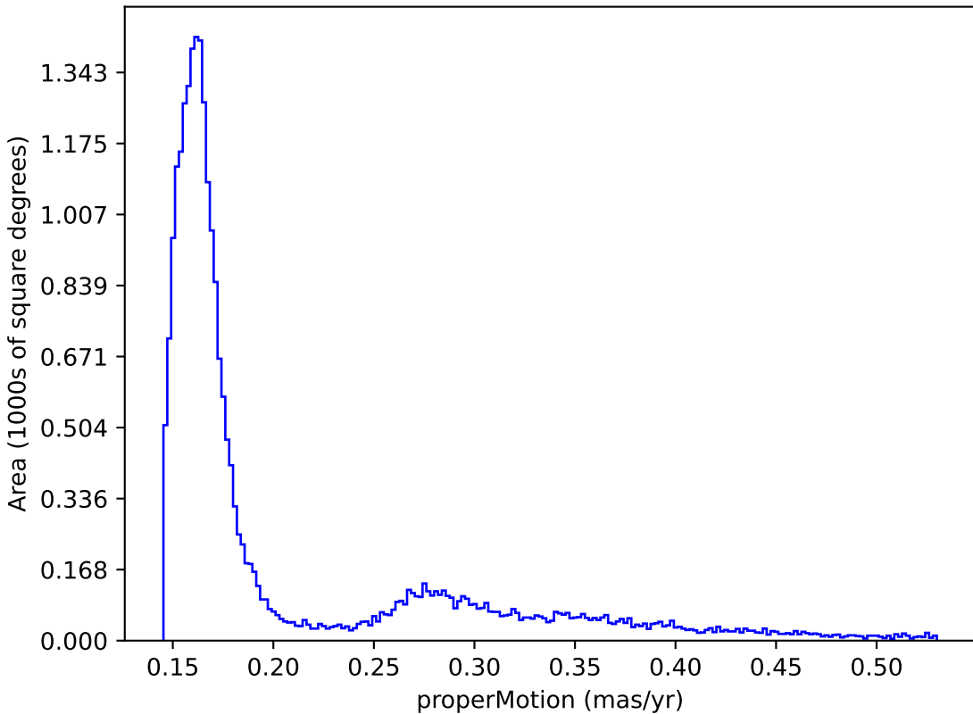
mw_roll_bulge_v3.3_10yrs : properMotion
