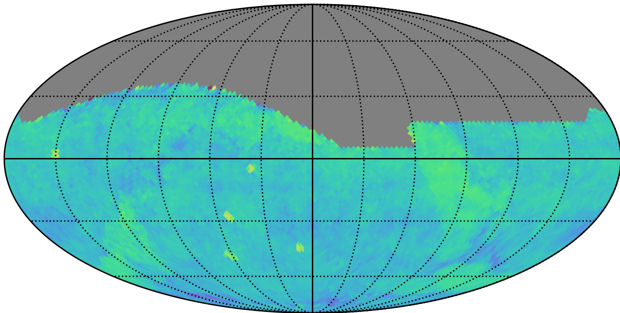
mw_roll_bulge_v3.3_10yrs (g or r or i): PairFraction
