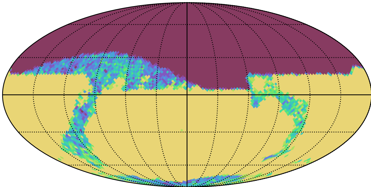
mw_roll_bulge_v3.3_10yrs r and night < 365: N year 1
