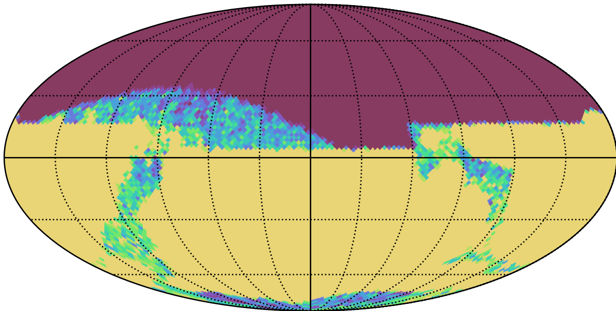
mw_roll_bulge_v3.3_10yrs i and night < 365: N year 1
