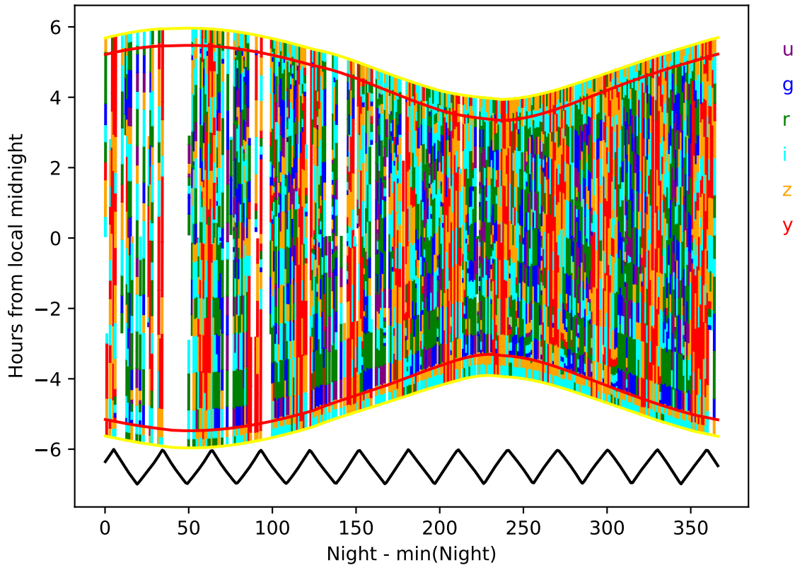
mw_roll_bulge_v3.3_10yrs year 6-7: Hourglass
