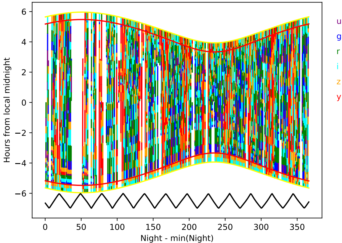
mw_roll_bulge_v3.3_10yrs year 2-3: Hourglass
