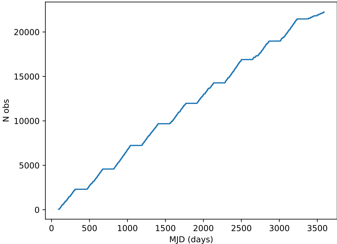
mw_roll_bulge_v3.3_10yrs note like DD:ECDFS%: Cumulative
