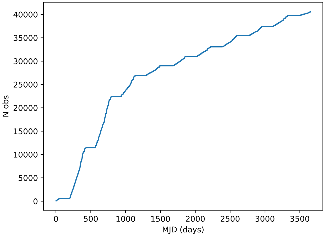
mw_roll_bulge_v3.3_10yrs note like DD:COSMOS%: Cumulative
