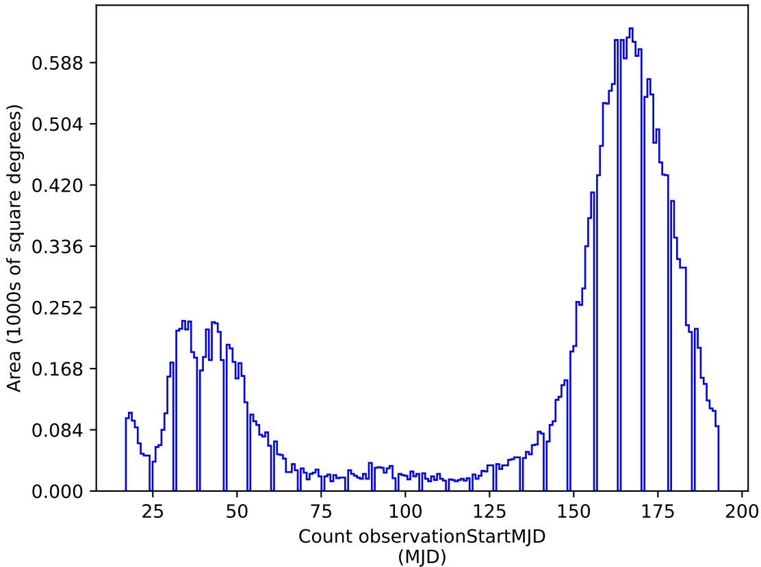
mw_roll_bulge_v3.3_10yrs z: Count observationStartMJD
