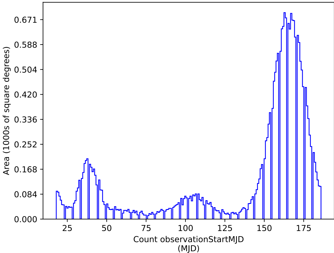
mw_roll_bulge_v3.3_10yrs y: Count observationStartMJD
