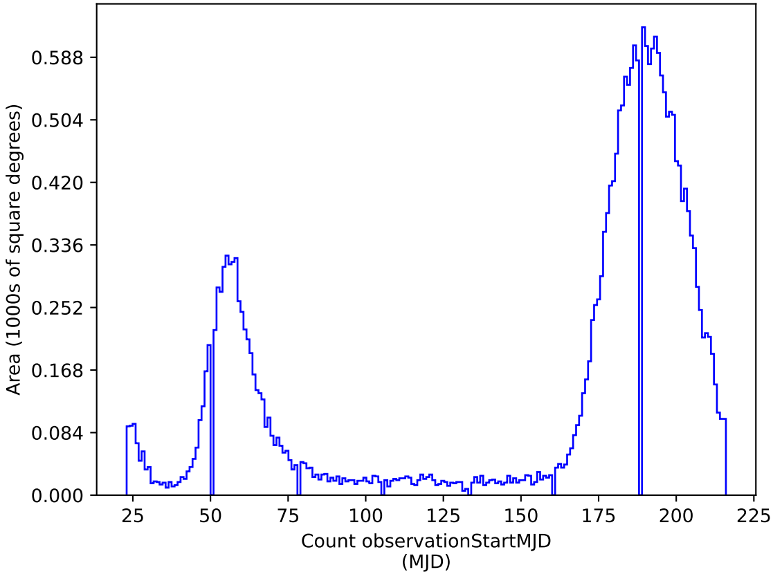
mw_roll_bulge_v3.3_10yrs i: Count observationStartMJD
