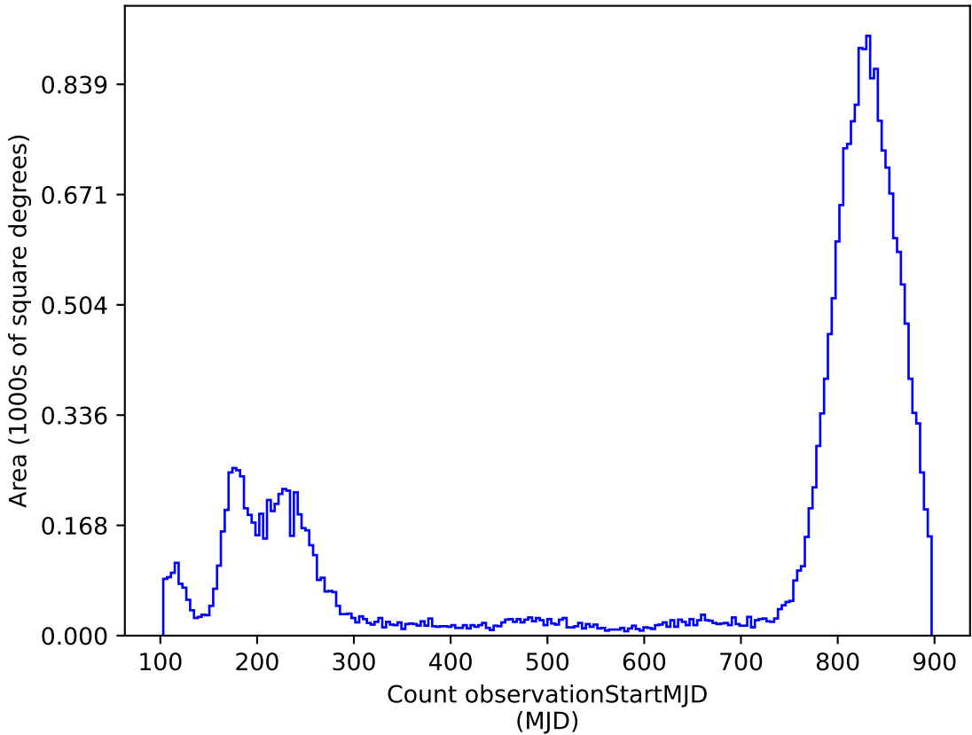
mw_roll_bulge_v3.3_10yrs : Count observationStartMJD
