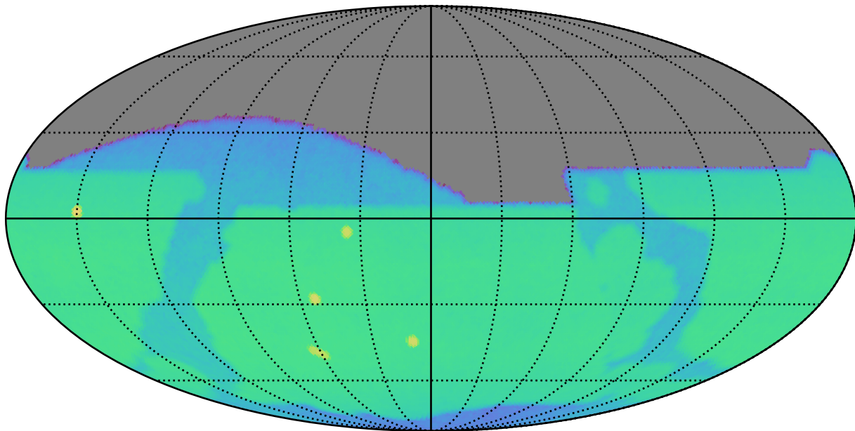
mw_roll_bulge_v3.3_10yrs z: CoaddM5
