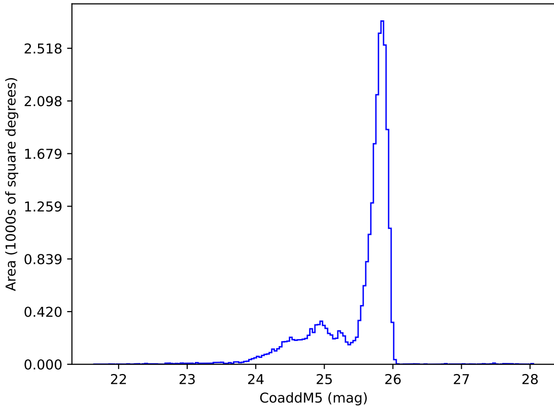
mw_roll_bulge_v3.3_10yrs z: CoaddM5
