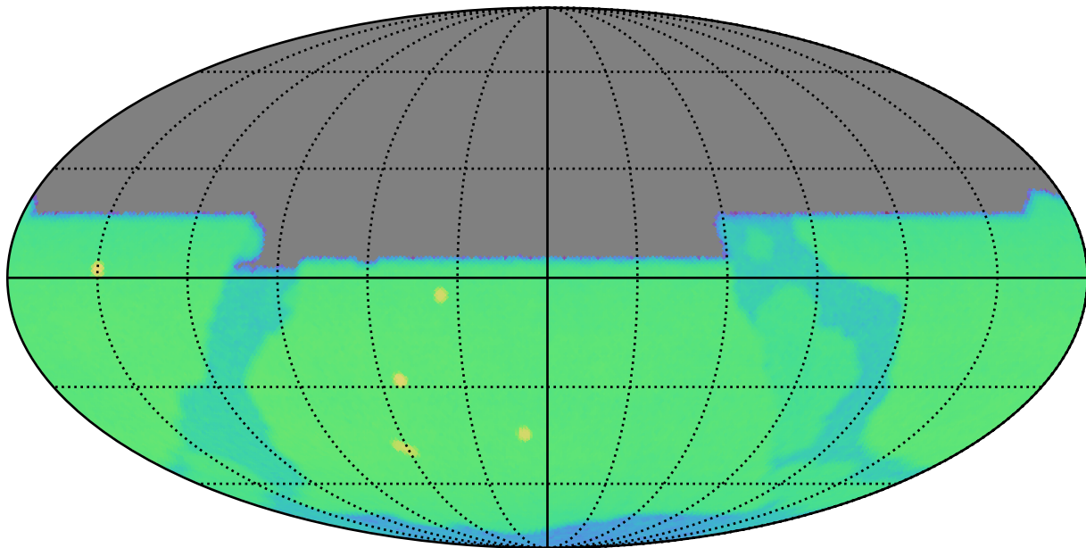
mw_roll_bulge_v3.3_10yrs y: CoaddM5
