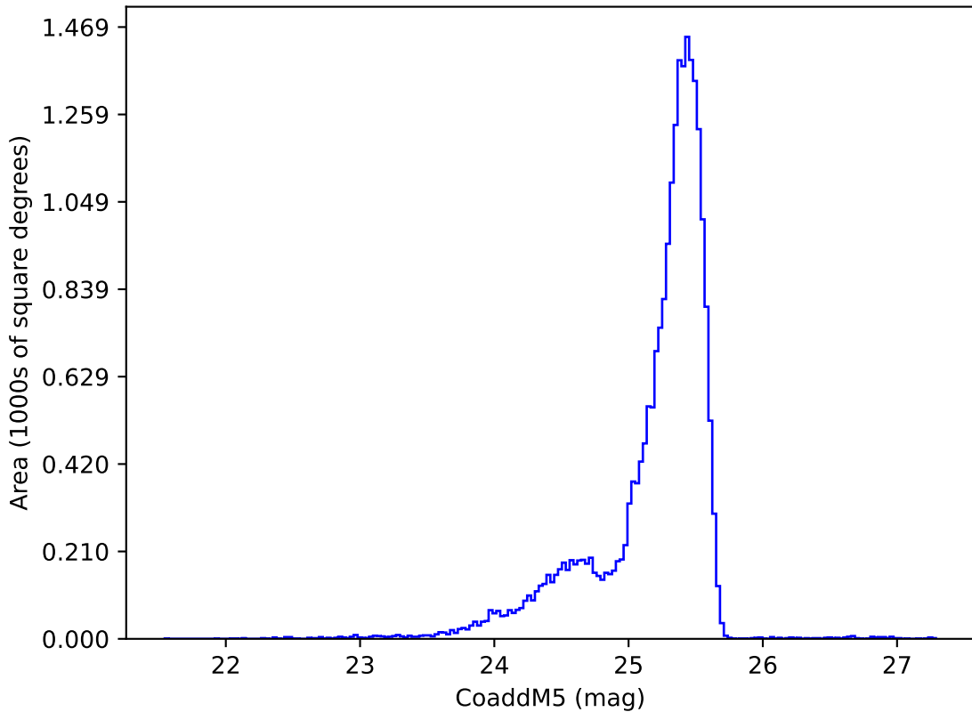
mw_roll_bulge_v3.3_10yrs u: CoaddM5
