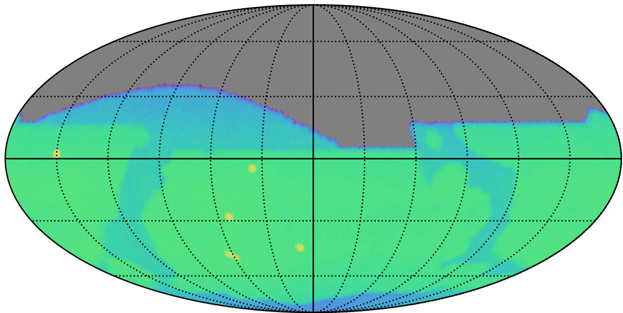
mw_roll_bulge_v3.3_10yrs i: CoaddM5
