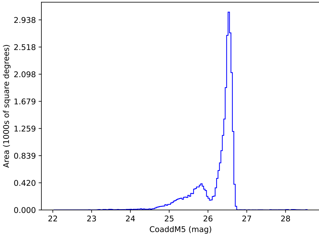
mw_roll_bulge_v3.3_10yrs i: CoaddM5
