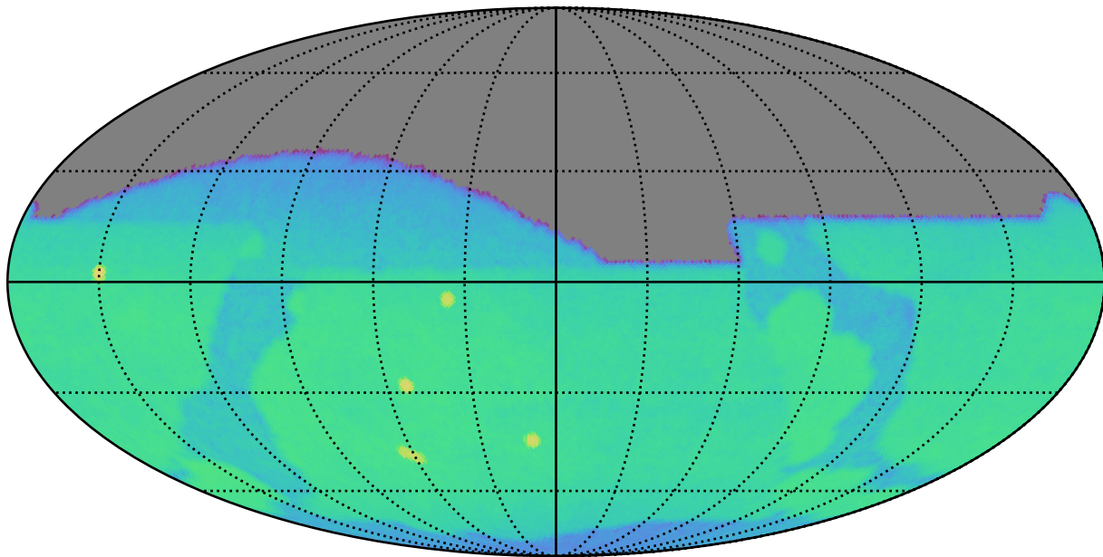
mw_roll_bulge_v3.3_10yrs g: CoaddM5
