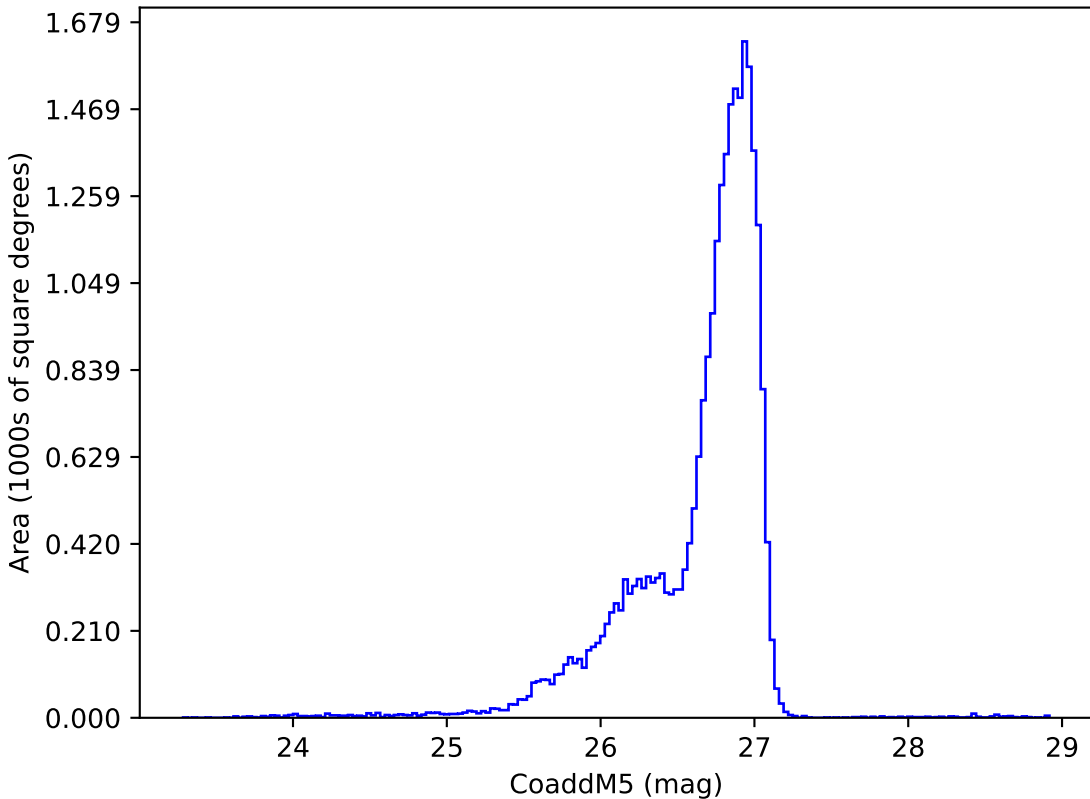
mw_roll_bulge_v3.3_10yrs g: CoaddM5
