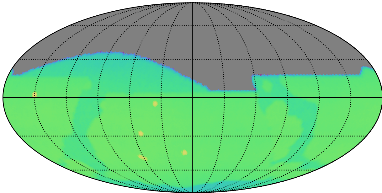
mw_roll_bulge_v3.3_10yrs : CoaddM5
