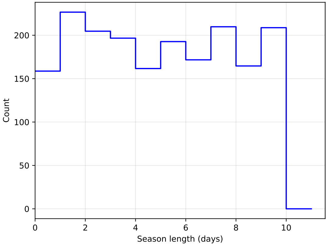
mw_roll_bulge_v3.3_10yrs DD:WFD all bands: SeasonLength
