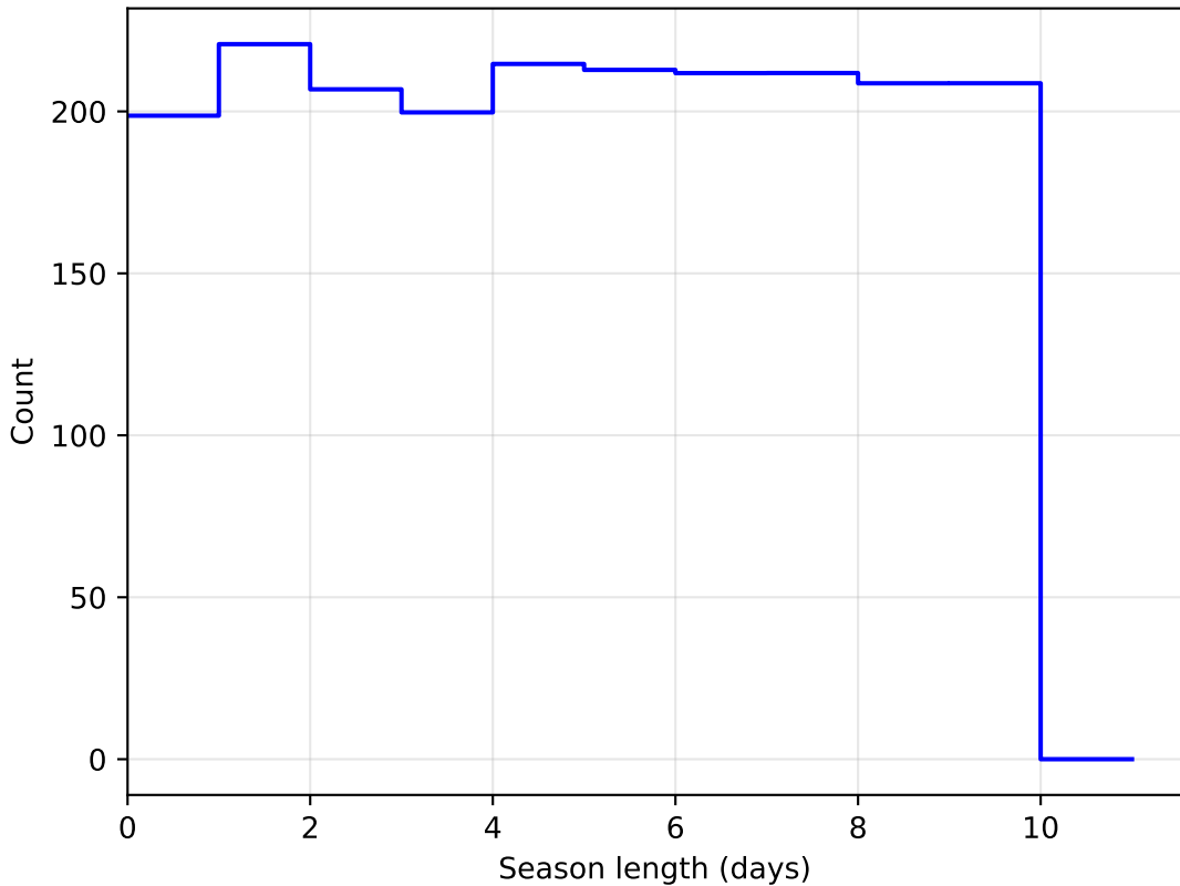
mw_roll_bulge_v3.3_10yrs DD:ELAISS1 all bands: SeasonLength
