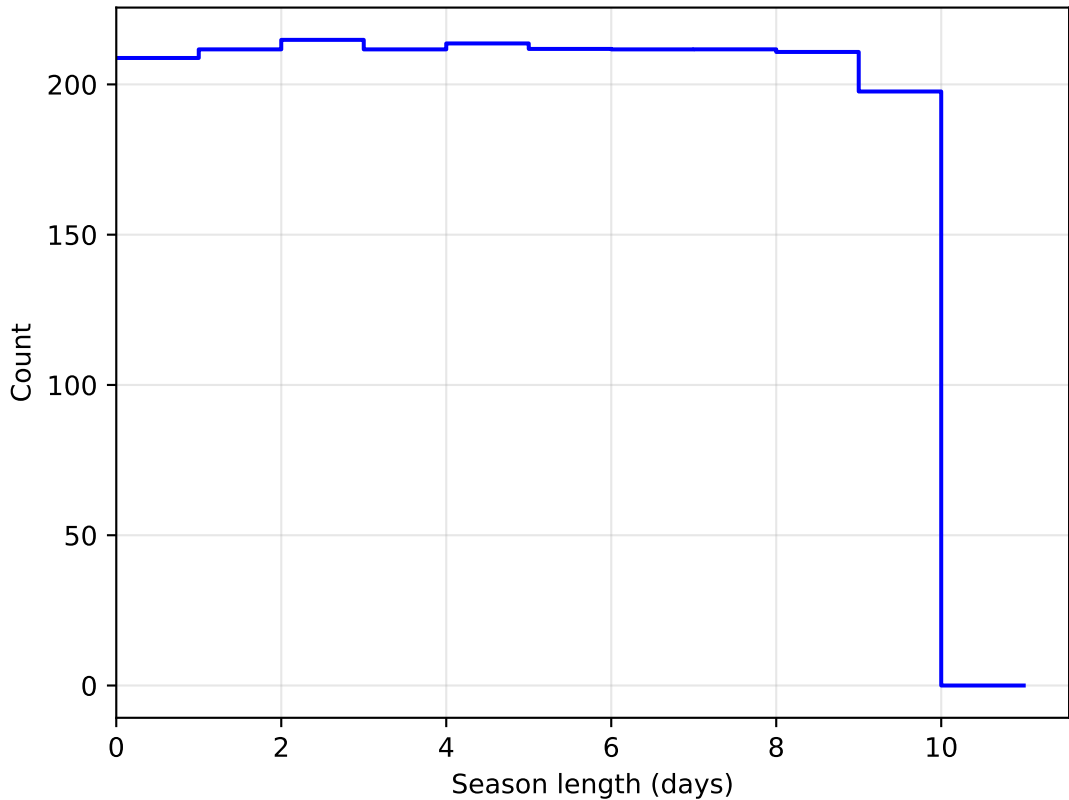
mw_roll_bulge_v3.3_10yrs DD:EDFS all bands: SeasonLength
