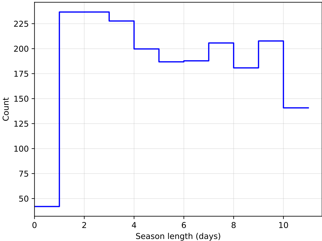
mw_roll_bulge_v3.3_10yrs DD: COSMOS all bands: SeasonLength
