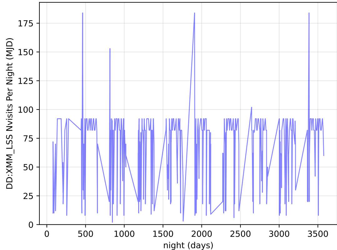
mw_roll_bulge_v3.3_10yrs all bands: DD:XMM_LSS Nvisits Per Night
