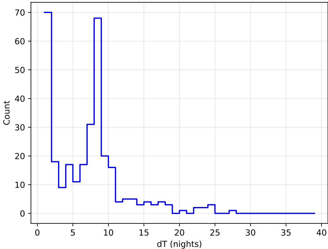
mw_roll_bulge_v3.3_10yrs all bands: DD:XMM_LSS Delta Nights Histogram
