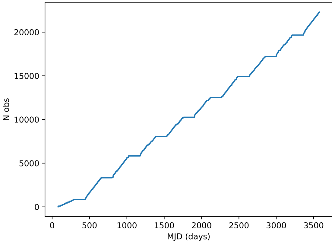
mw_roll_bulge_v3.3_10yrs all bands: DD:XMM_LSS Cumulative NVisits
