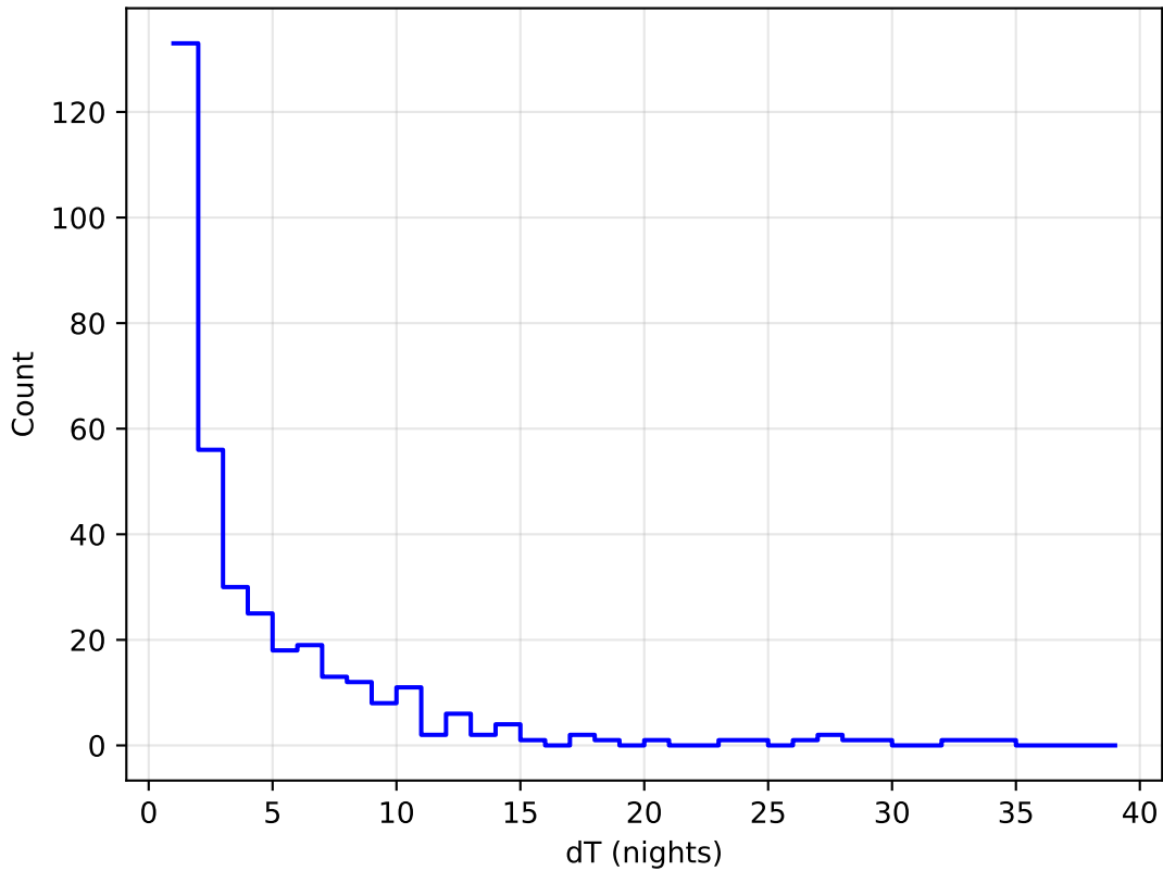
mw_roll_bulge_v3.3_10yrs all bands: DD:WFD Delta Nights Histogram
