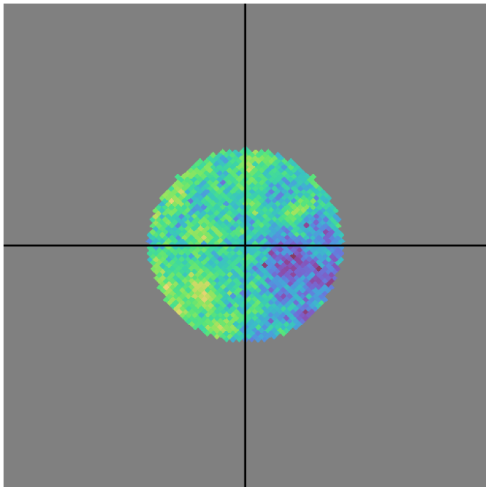
mw_roll_bulge_v3.3_10yrs g band: DD:WFD CoaddM5
