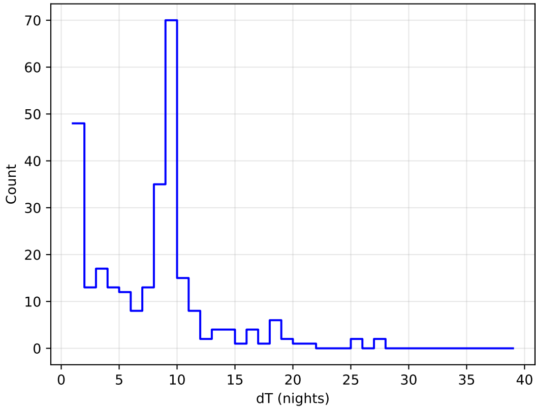
mw_roll_bulge_v3.3_10yrs all bands: DD:ELAISS1 Delta Nights Histogram
