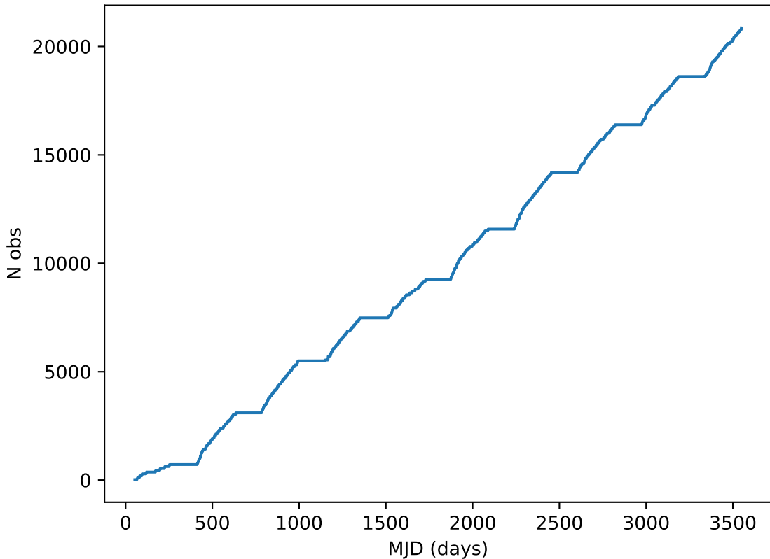
mw_roll_bulge_v3.3_10yrs all bands: DD:ELAISS1 Cumulative NVisits
