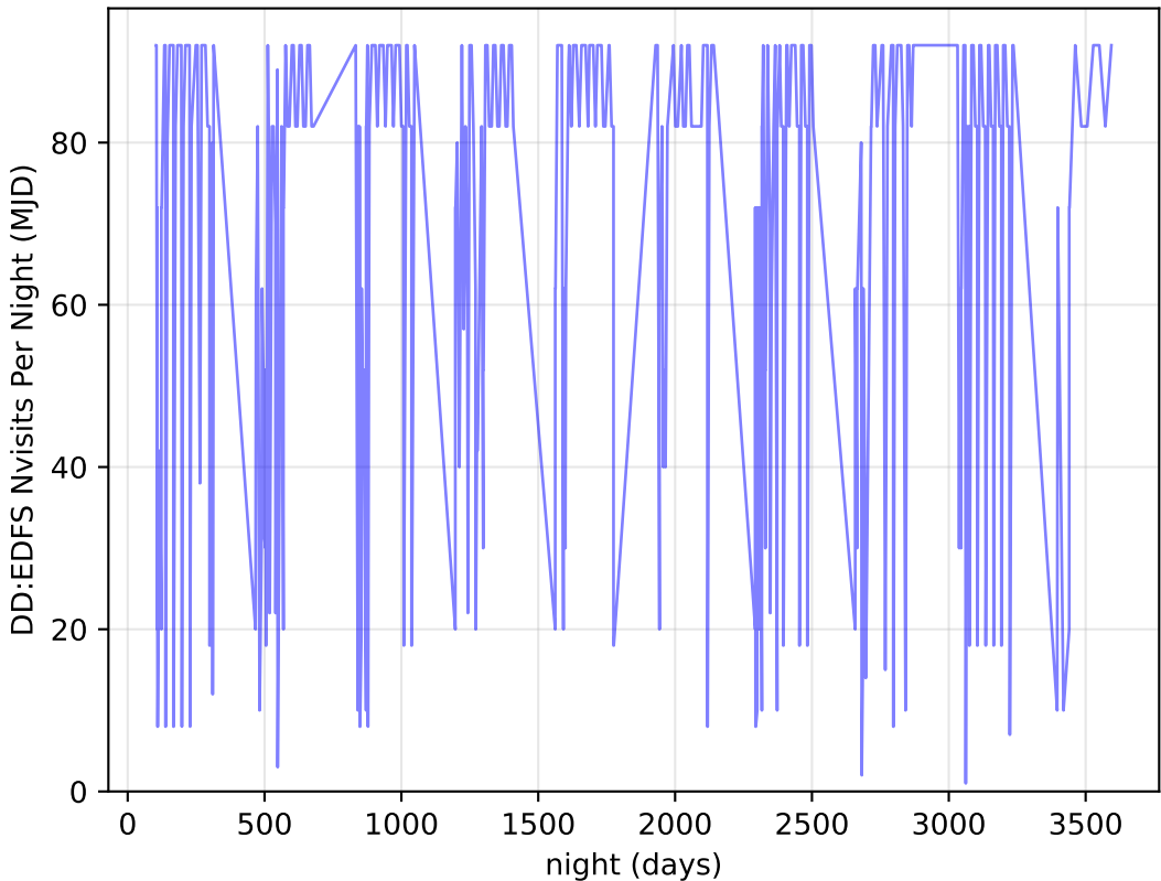
mw_roll_bulge_v3.3_10yrs all bands: DD:EDFS Nvisits Per Night
