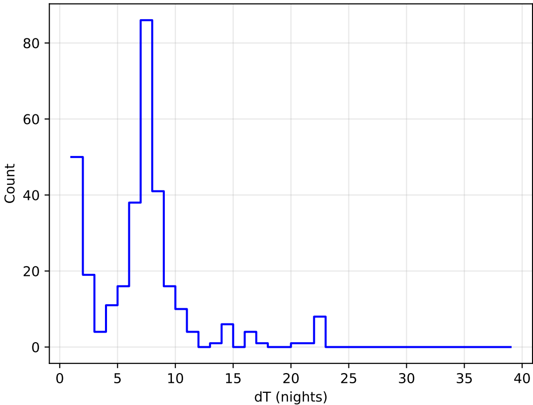
mw_roll_bulge_v3.3_10yrs all bands: DD:EDFS Delta Nights Histogram
