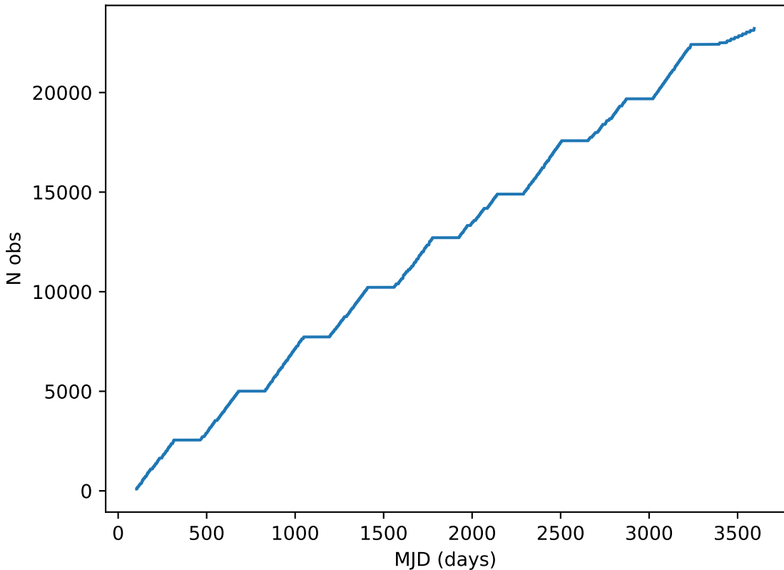
mw_roll_bulge_v3.3_10yrs all bands: DD:EDFS Cumulative NVisits
