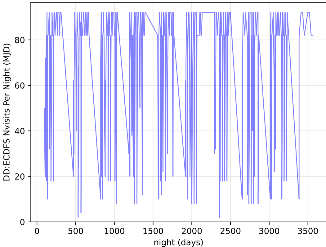
mw_roll_bulge_v3.3_10yrs all bands: DD:ECDFS Nvisits Per Night
