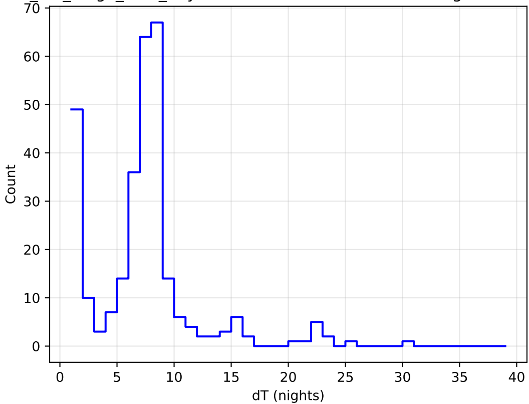
mw_roll_bulge_v3.3_10yrs all bands: DD:ECDFS Delta Nights Histogram
