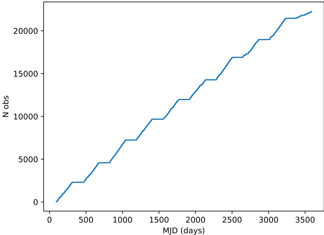
mw_roll_bulge_v3.3_10yrs all bands: DD:ECDFS Cumulative NVisits
