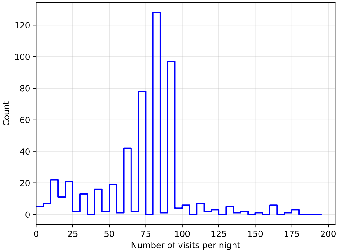
mw_roll_bulge_v3.3_10yrs all bands: DD:COSMOS NVisitsPerNight
