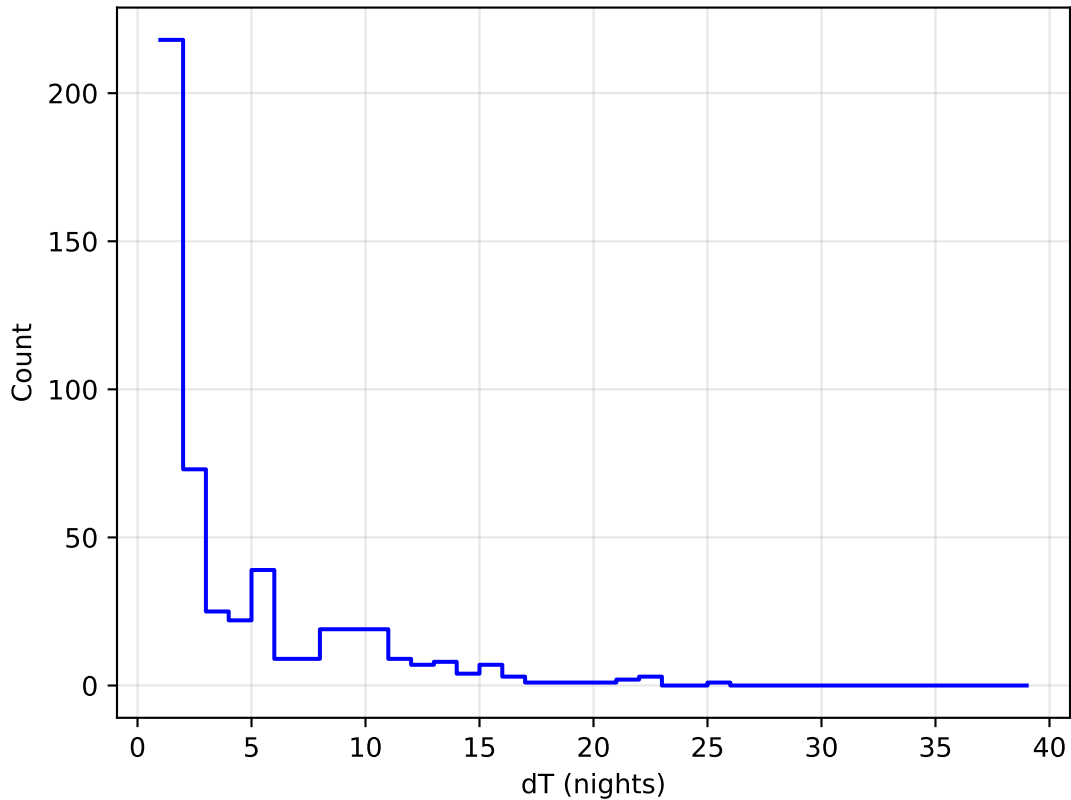
mw_roll_bulge_v3.3_10yrs all bands: DD: COSMOS Delta Nights Histogram
