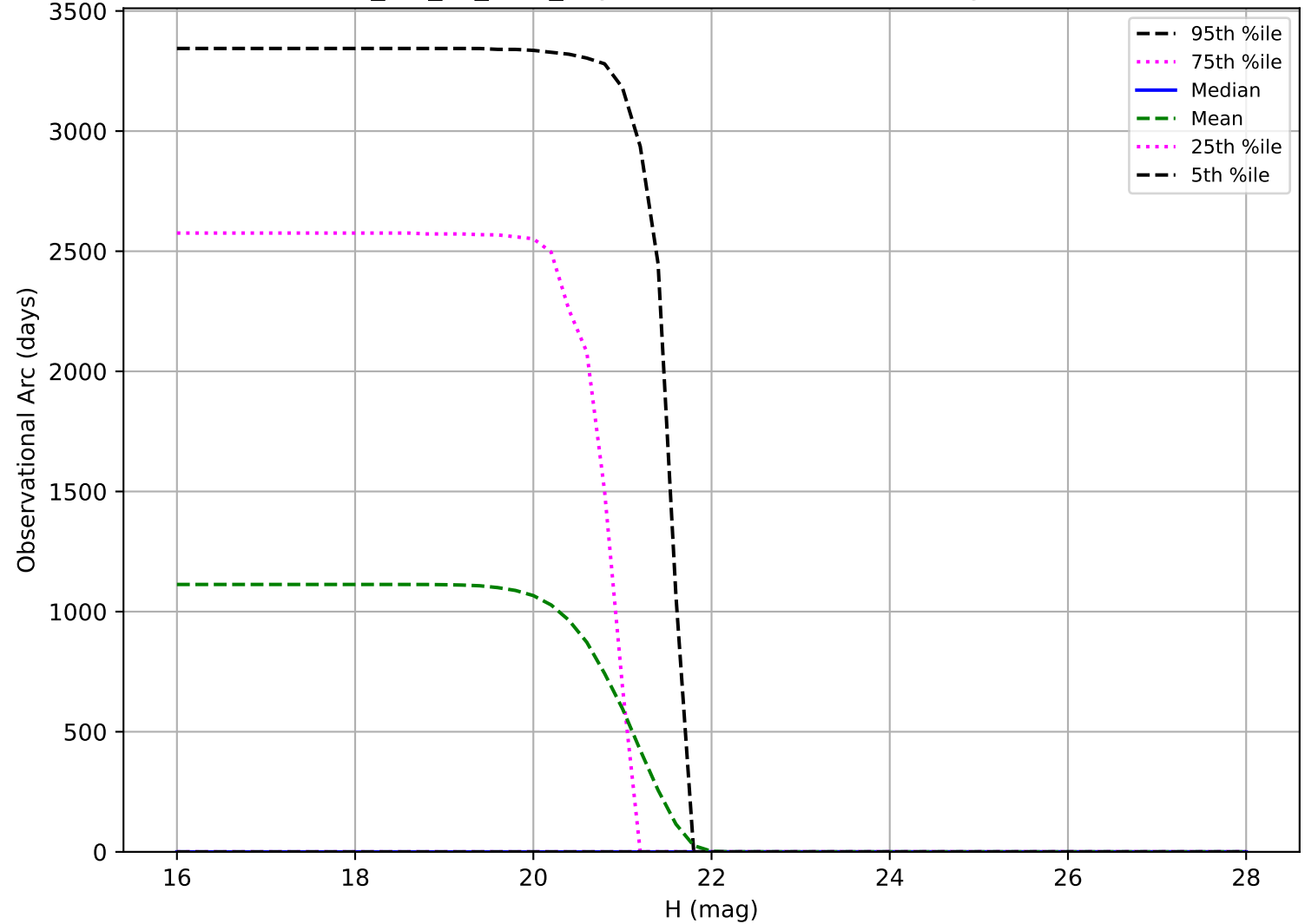
mw_roll_all_v3.3_10yrs: Observational Arc Length Vatira
