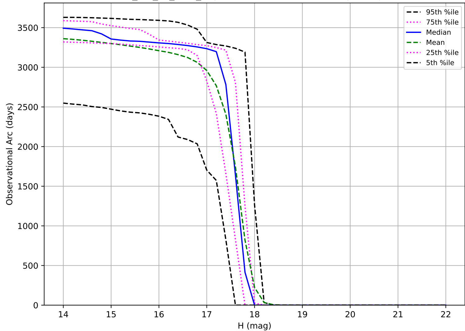
mw_roll_all_v3.3_10yrs: Observational Arc Length Trojan
