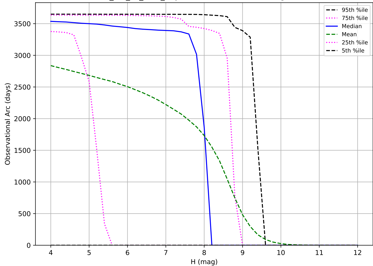
mw_roll_all_v3.3_10yrs: Observational Arc Length TNO
